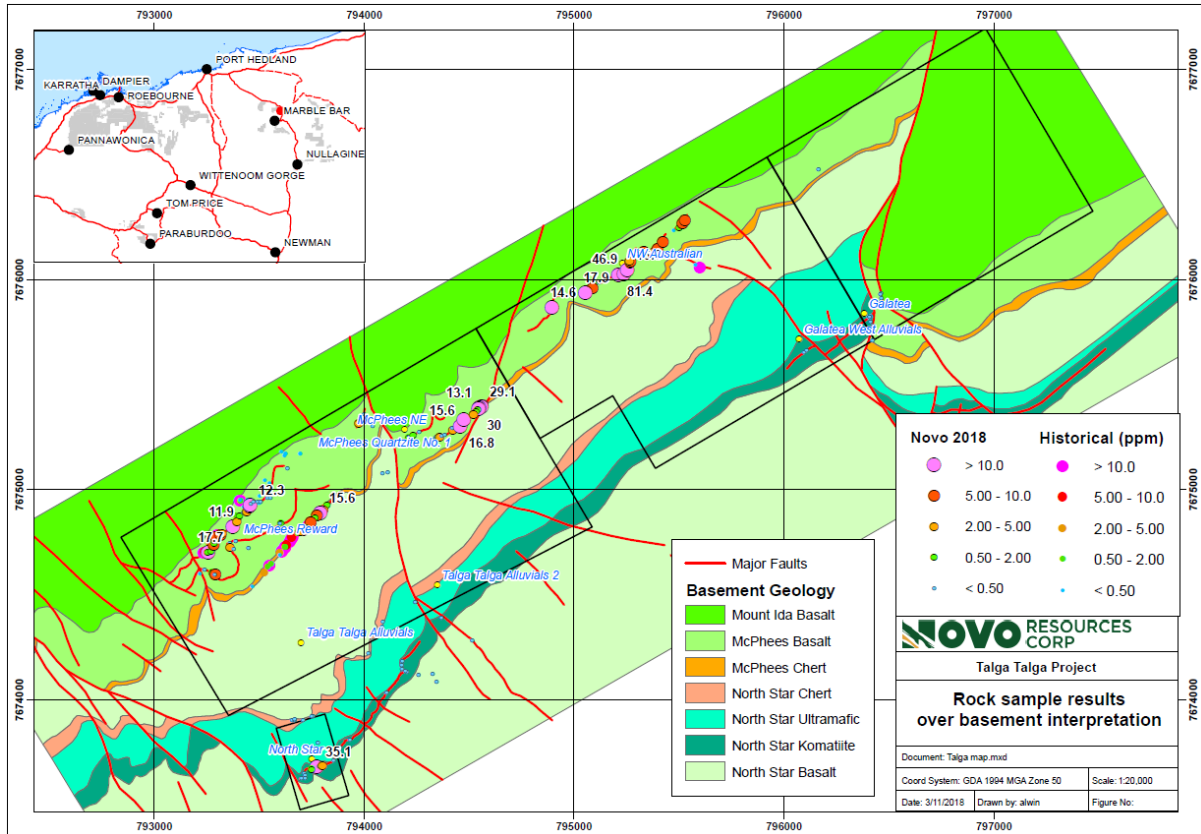
(Figure 2 – Geologic map of the Talga Talga project. Spot rock chip sampling has defined a three kilometer long corridor of mineralized structures extending from McPhee’s Reward in the southwest to NW Australian in the northeast.)
