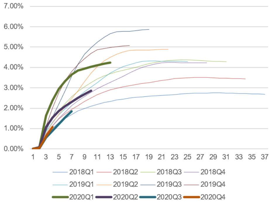
DPD 30+/GMV by performance windows
