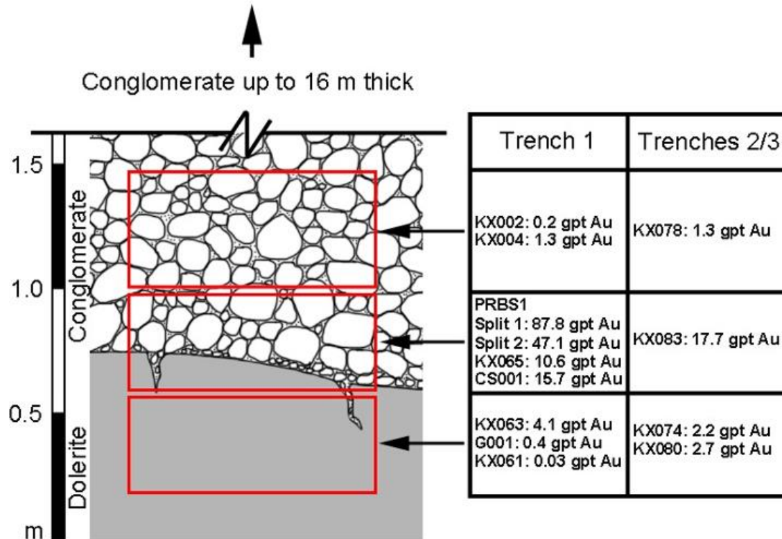
( Figure 5: Schematic section through the basal conglomerate section and footwall dolerite at Purdy's Reward. Red boxes show the location of bulk samples taken from the lithologic section. Results in the table on the right show respective grades returned from bulk samples from trenches 1, 2 and 3. These bulk samples each weigh approximately 300 kg, small compared to the recommended minimum sample size of five tonnes. Highest gold grades are situated in the basal part of the section. Gold is also present in overlying conglomerates, but Novo believes large samples will be necessary to better evaluate grades in this lower grade material. Gold in samples of the footwall dolerite may be coming from cracks and crevasses along the contact. Samples KX078, CS001 and KX083 were first reported in a news release dated December 21, 2017. Samples PRBS1 Split 1 and Split 2 were first reported in a news release dated August 8, 2017.)
