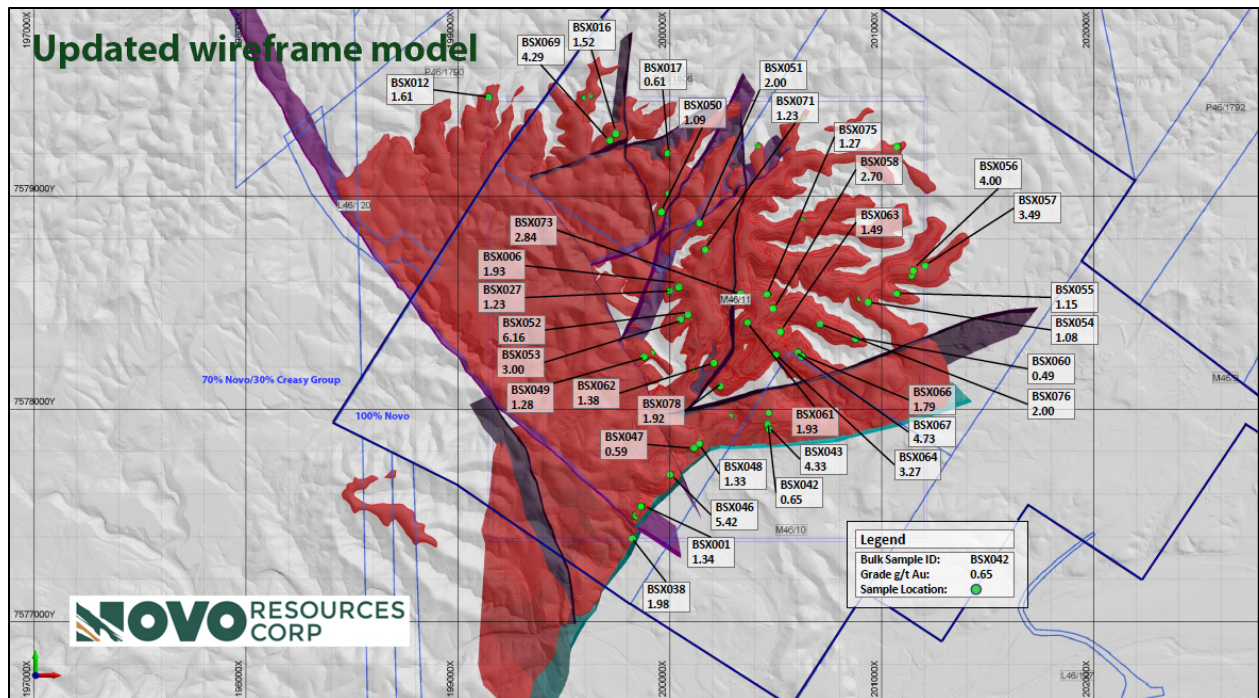
(Figure 2 – Plan view of the updated wireframe model of gold-bearing conglomerate deposits [red] at Beatons Creek showing the locations of 2-tonne bulk sample sites [green dots]. Green dots without labels are samples that have not yet returned from the laboratory. Faults [blues and black] define discrete domains.)
