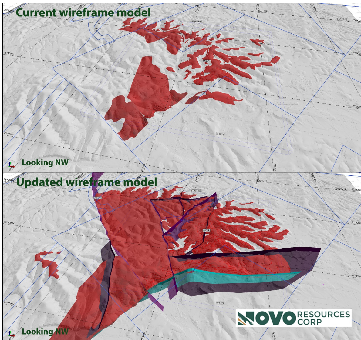
(Figure 1 – Oblique views of the current and updated wireframe models of gold-bearing conglomerate deposits [red] at Beatons Creek. Note the array of faults [blues and black] modeled in the lower image that define discrete domains.)
