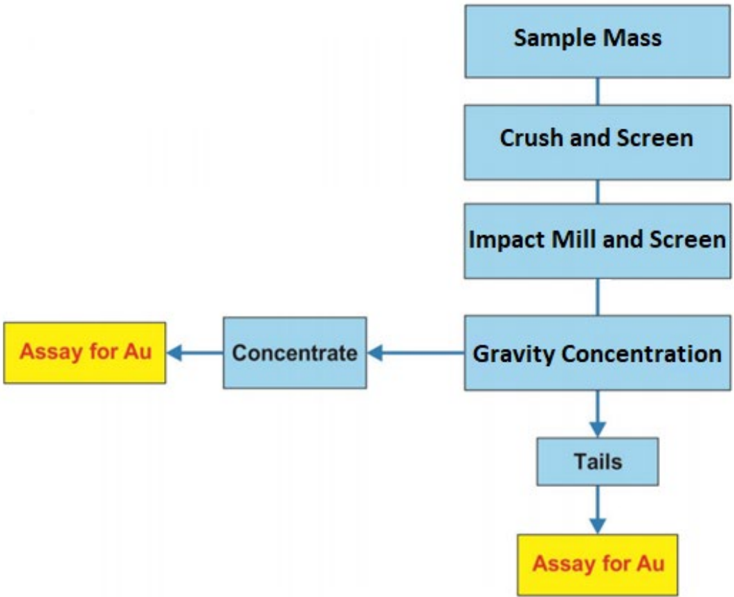
(Figure 5 – Flow chart for processing 2-tonne bulk samples from Beatons Creek. Concentrates are assayed in the entirety whereas tails are split and assayed.)
