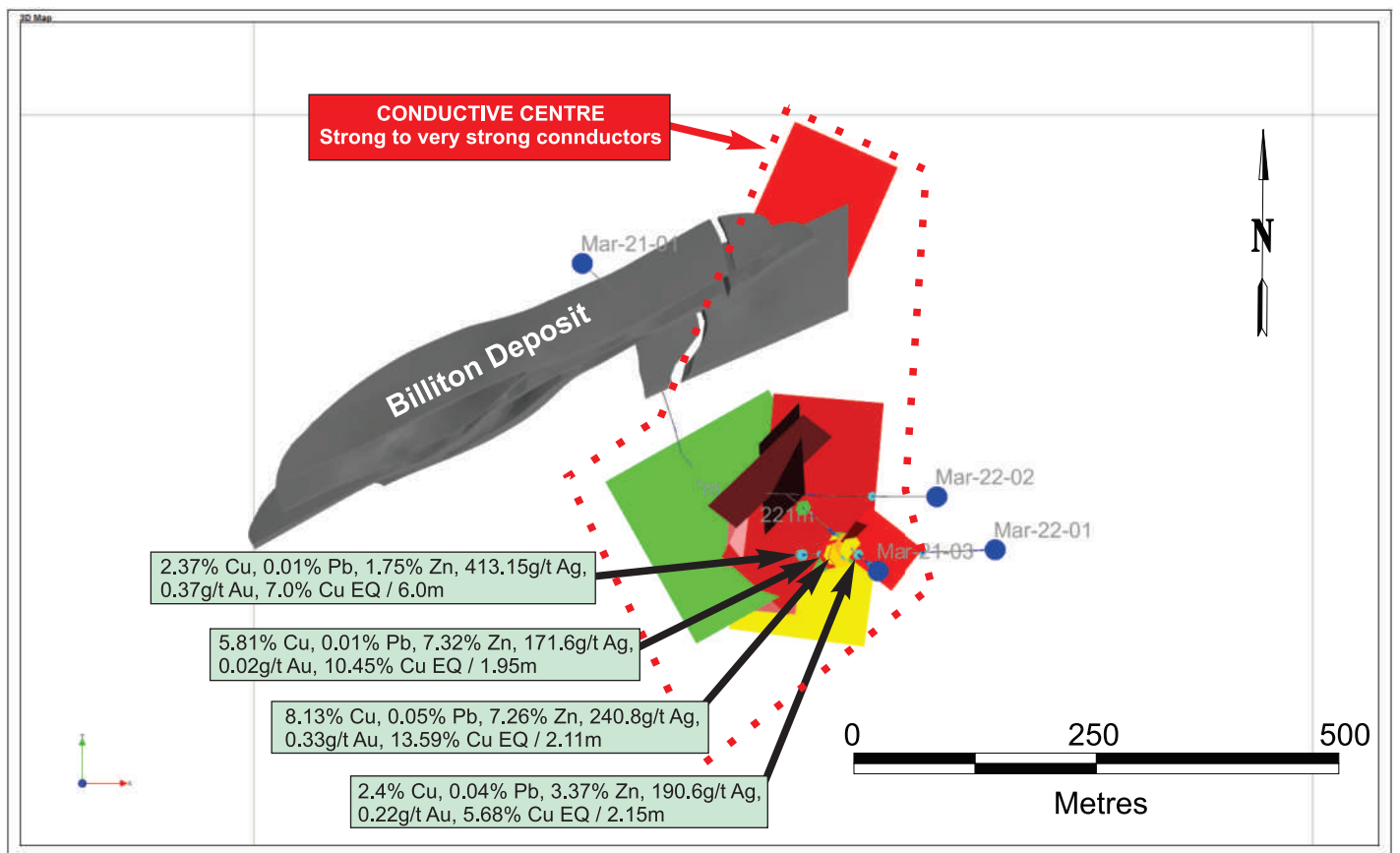
Figure 1A: Plan map showing the conductive centre relative to the high-grade intercepts in Mar-22-01 and the Billiton deposit
