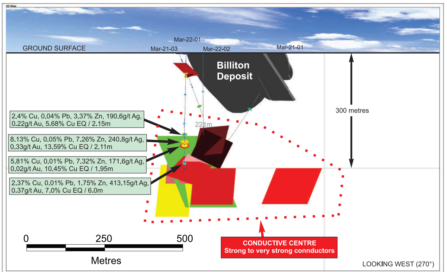
Figure 1B: 3D depiction (looking west) illustrating the conductive centre relative to the high-grade intercepts in Mar-22-01 and the Billiton deposit.
