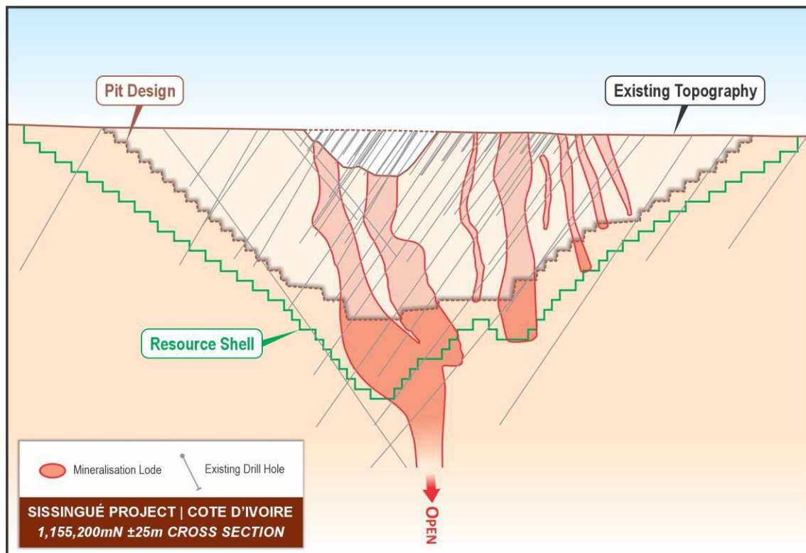
Figure 6: Cross section of Bagoé Ore Reserve pit design with Mineral Resource shell
