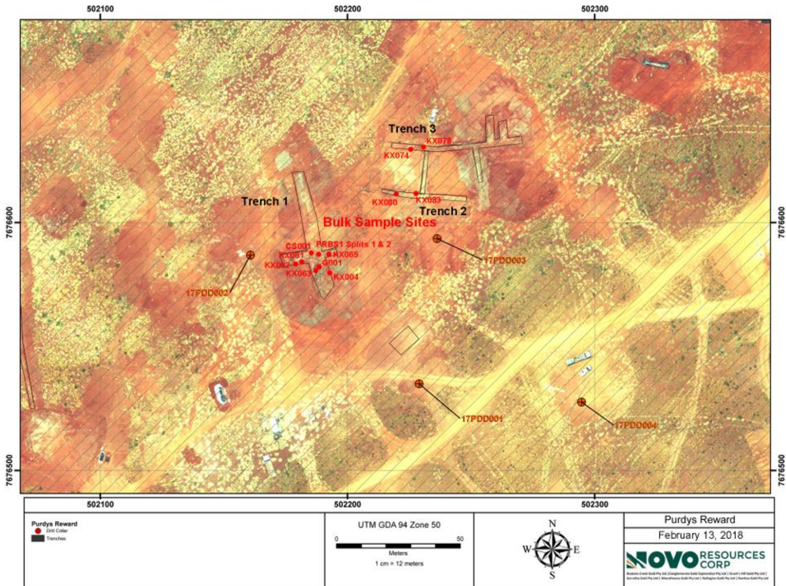
(Figure 6: Plan map showing the location of Trenches 1, 2 and 3. Bulk sample locations are also highlighted. Drill holes shown were discussed in a news release dated December 21, 2017.)
