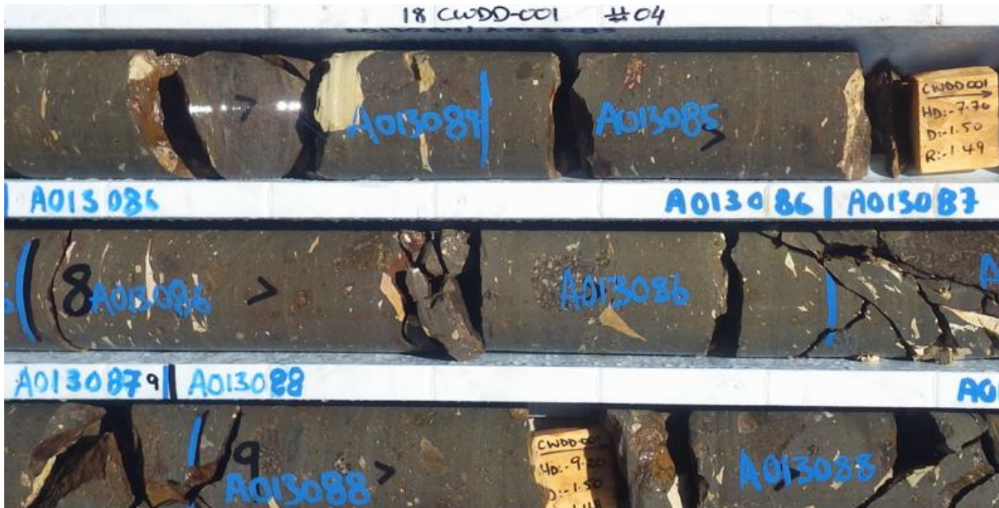
( Figure 7: Marker unit that sits beneath the newly discovered gold-bearing conglomerate. PQ core is from diamond drill hole CWDD-001. Lite colored shards, possibly lapilli, occur in a dark ashy matrix. This unit may prove useful in helping establish continuity of the conglomerate above.)
