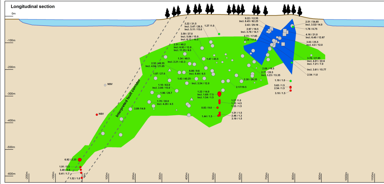
UTM NAD 83 Zone 18 Figure 1 - Longitudinal section June 5, 2019 press release
