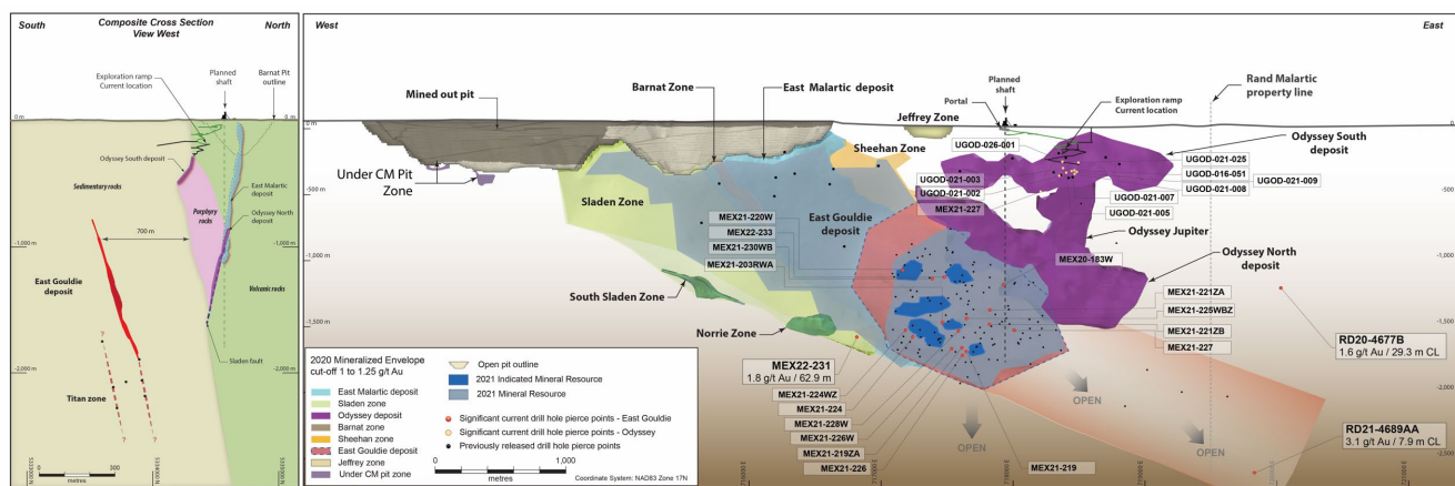
Figure 1 : Mine Canadian Malartic – coupe longitudinale
