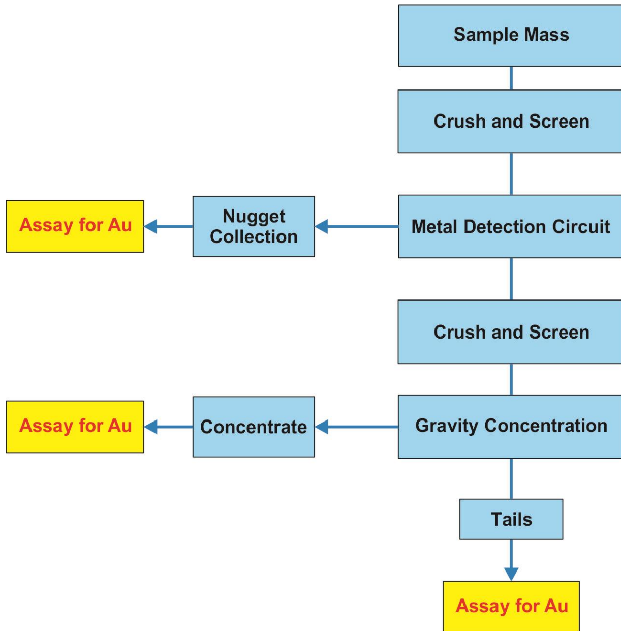
(Figure 3 – SGS Bulk Sample flowsheet)
