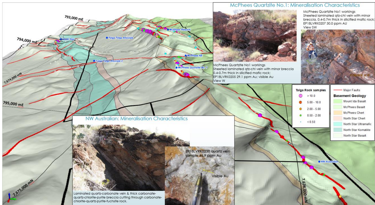
( Figure 3 – Oblique view looking southwest along a three kilometer corridor of mineralized structures extending from NW Australian to McPhee’s Reward. Inset photographs show examples of gold-bearing quartz veins. Dips are generally 35-40 degrees northwest.)
