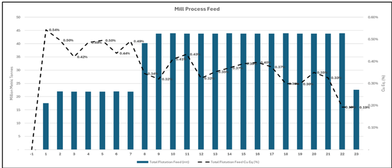
Figure 4: Mill Production Schedule
