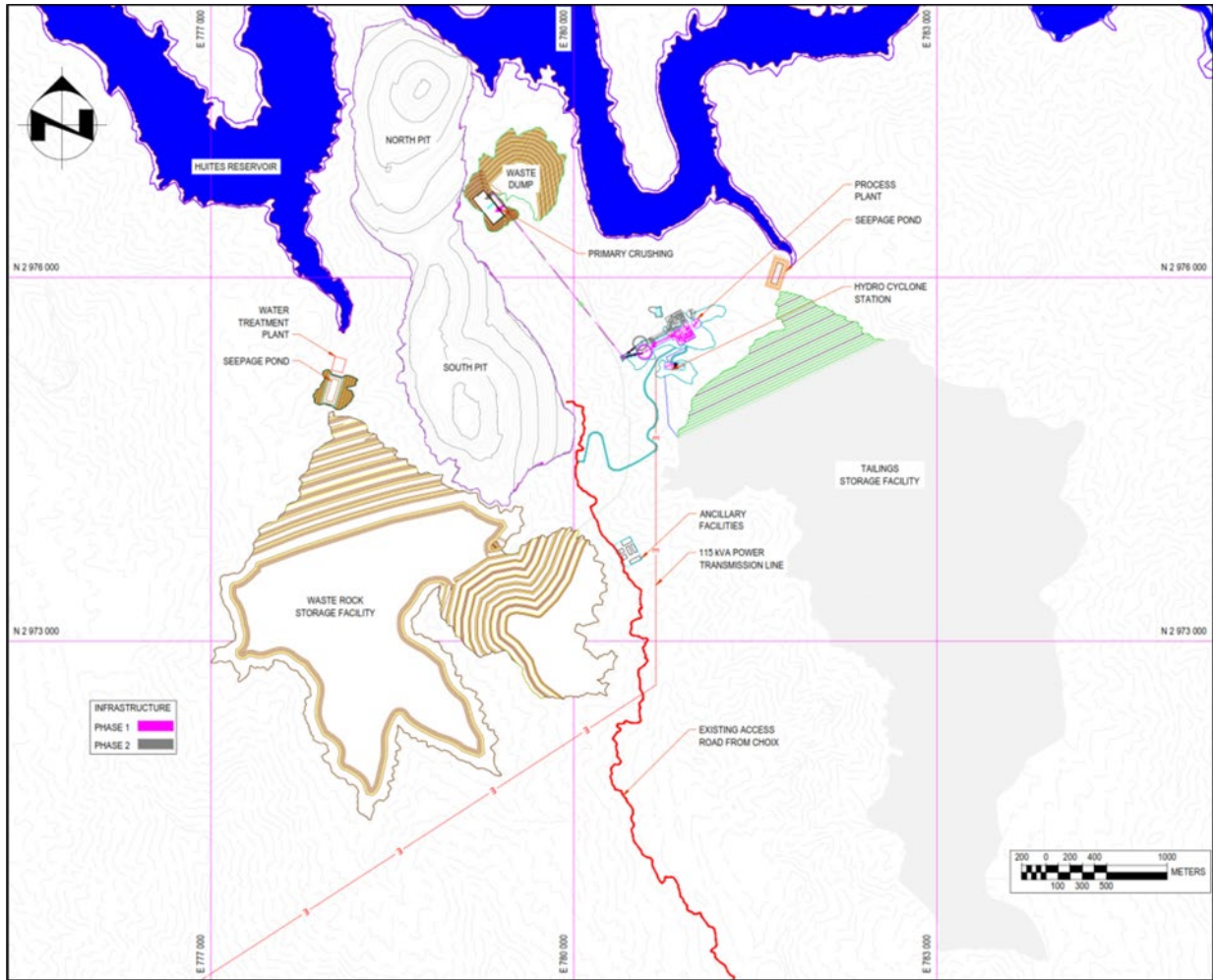
Figure 6: Mine Infrastructure, Pits, Process Plant Layout, Tailings and Waste Rock Storage Facilities
