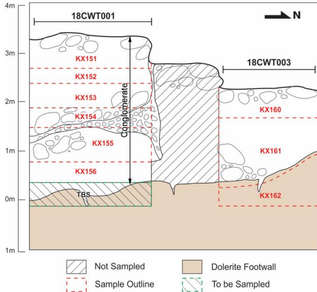
(Figure 1: Illustration showing samples taken from the basal bouldery conglomerate exposed in trenches 18CWT001 and 18CWT003 at the Powerline showing at Comet Well. Dip of the units is to the left. Each bulk sample is collected from a 2 x 2 m subhorizontal panel at least 0.3 m thick. Samples weigh approximately 5 tonnes or greater. Footwall dolerite is also routinely sampled. Novo plans to use bulk samples such as these to assess the grade of the conglomerate package.)
