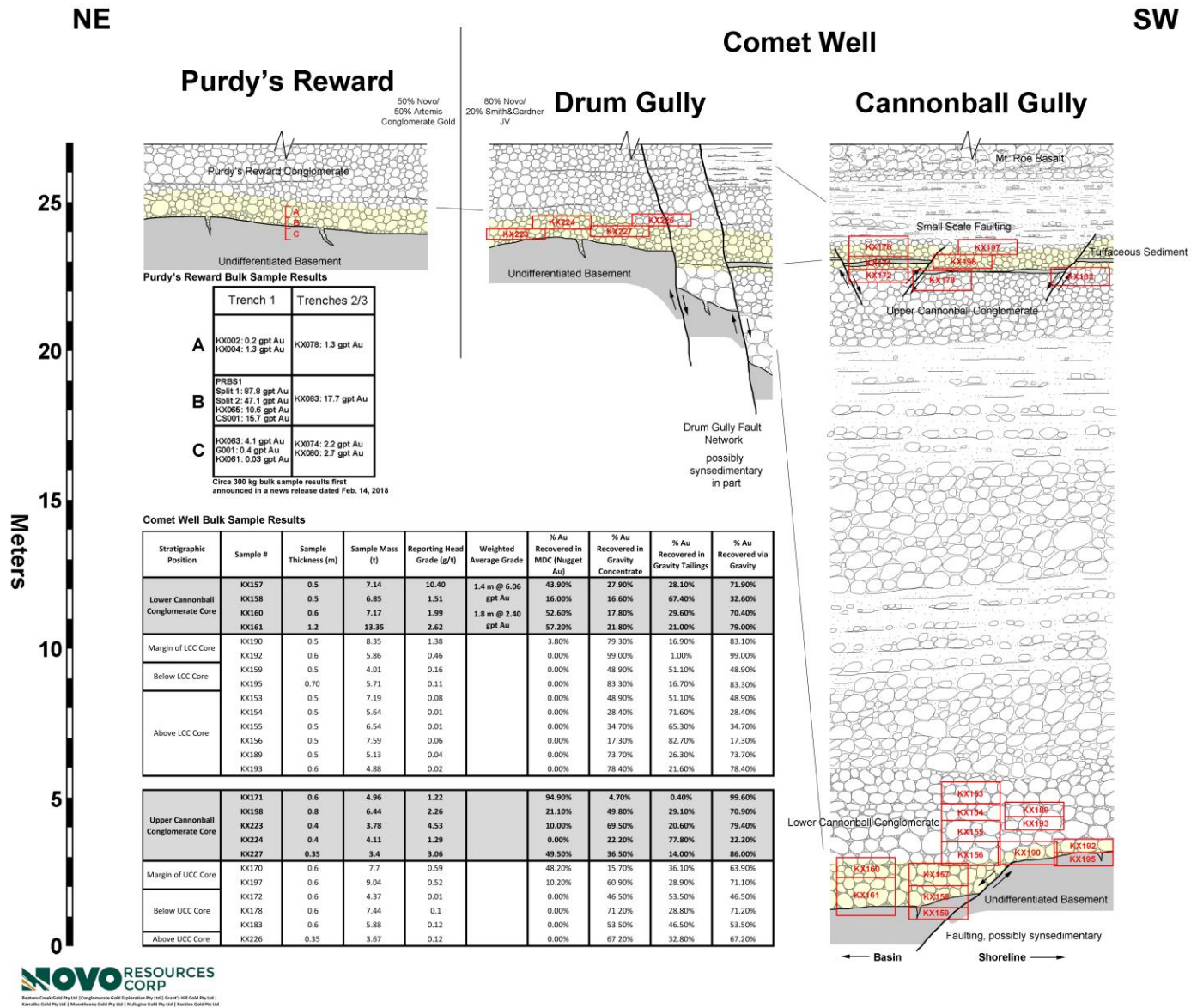
(Figure 2 – Schematic stratigraphic sections from Cannonball Gully, Drum Gully and Purdy's Reward showing the position of bulk samples and the two gold-bearing conglomerate units. The bounds of gold-bearing conglomerates are not readily identifiable by eye, therefore bulk sampling encompassed sections of conglomerate above and below each respective gold-bearing unit in order to better constrain their limits.)
