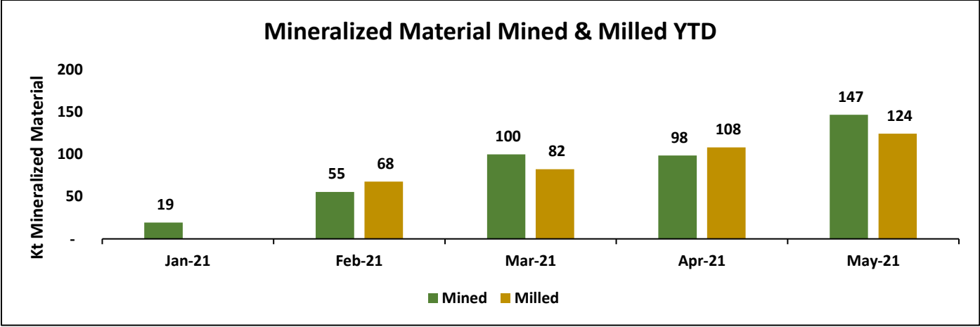
(Figure 2: Mineralized material mining and milling rates for the Nullagine Gold Project to date.)
