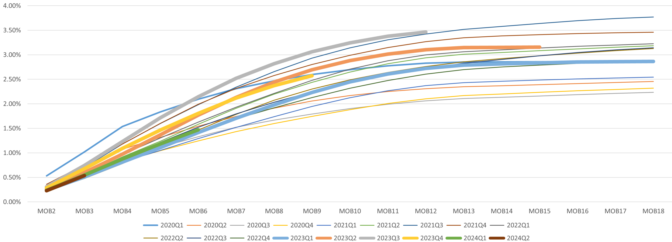
30 Day+ Delinquency Rate by Vintage
