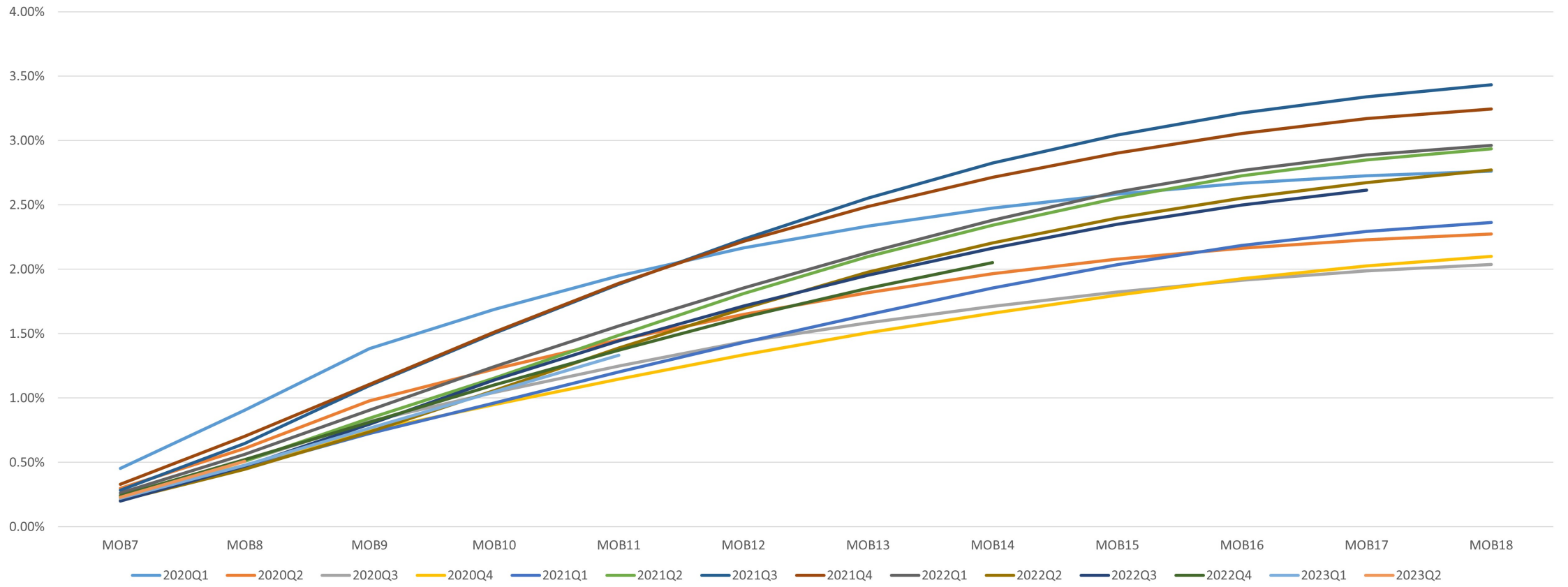
180 Day+ Delinquency Rate by Vintage
