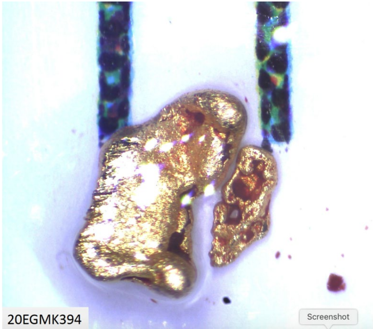
(Figure 2: Example of gold grains from a MAK sample collected at Paradise. Black lines denote 1 mm. The particle on the left is considered a nugget given it is larger than 1 mm. Such gold resembles gold discovered in a swale on the Egina mining lease in 2020. This is a concentrated sample of selected material and is not necessarily representative of mineralization hosted on the Egina property.)
