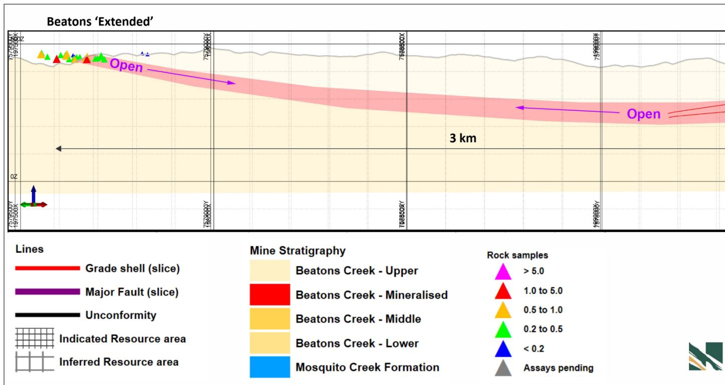
( Figure 2: Cross sectional view of the mineralized sequence at Beatons Creek west of the Grant's Hill fault.)
